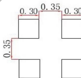
P1.25 推荐焊盘尺寸 Recommended Soldering Pad
