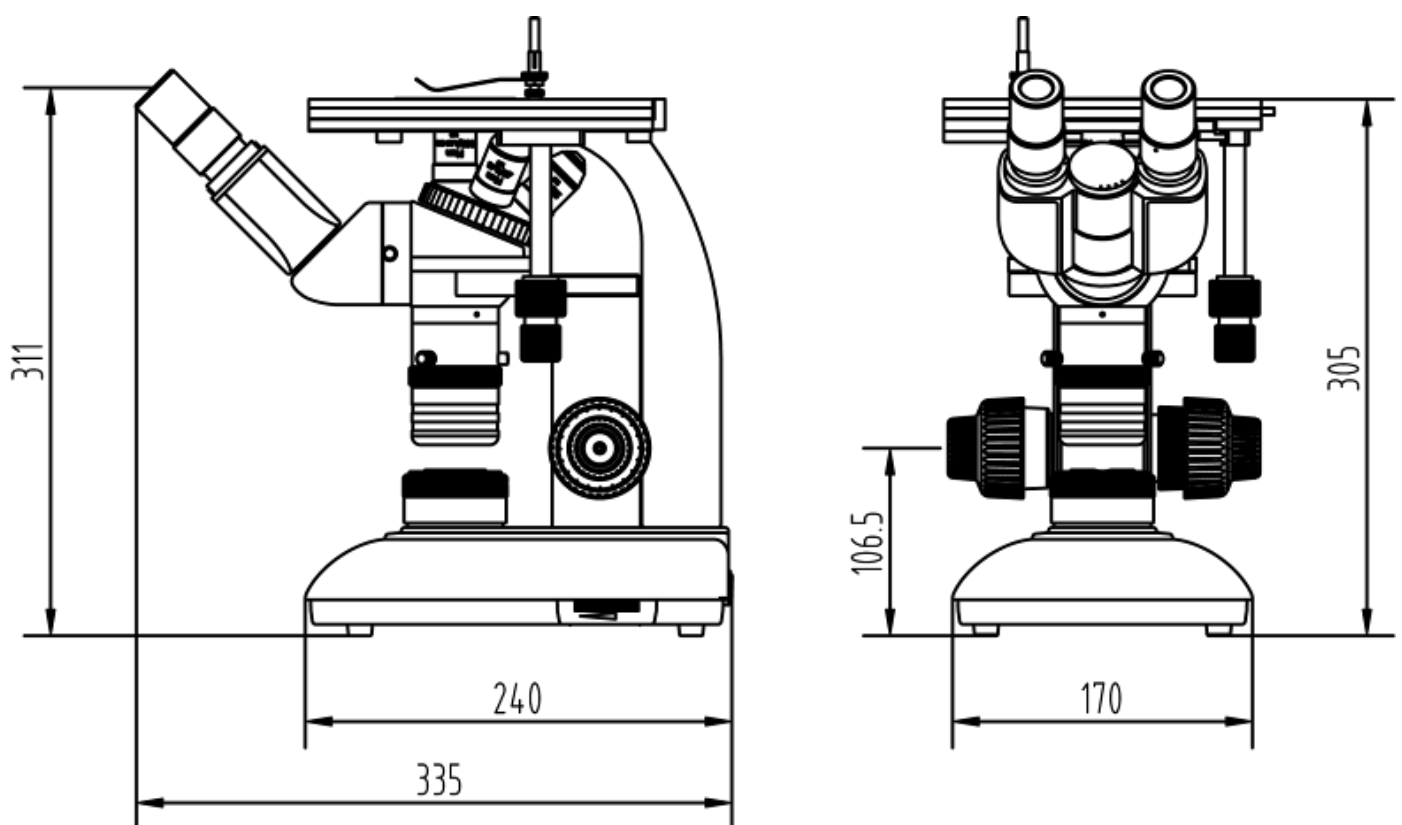
A13.2602 Inverted Metallurgical Microscope Size(mm)
