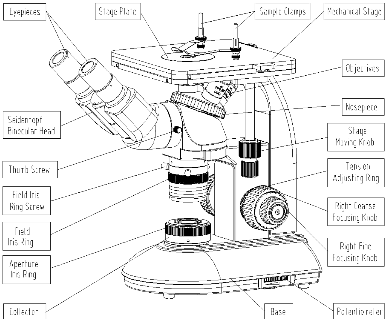
A13.2602-B General Layout Diagram
