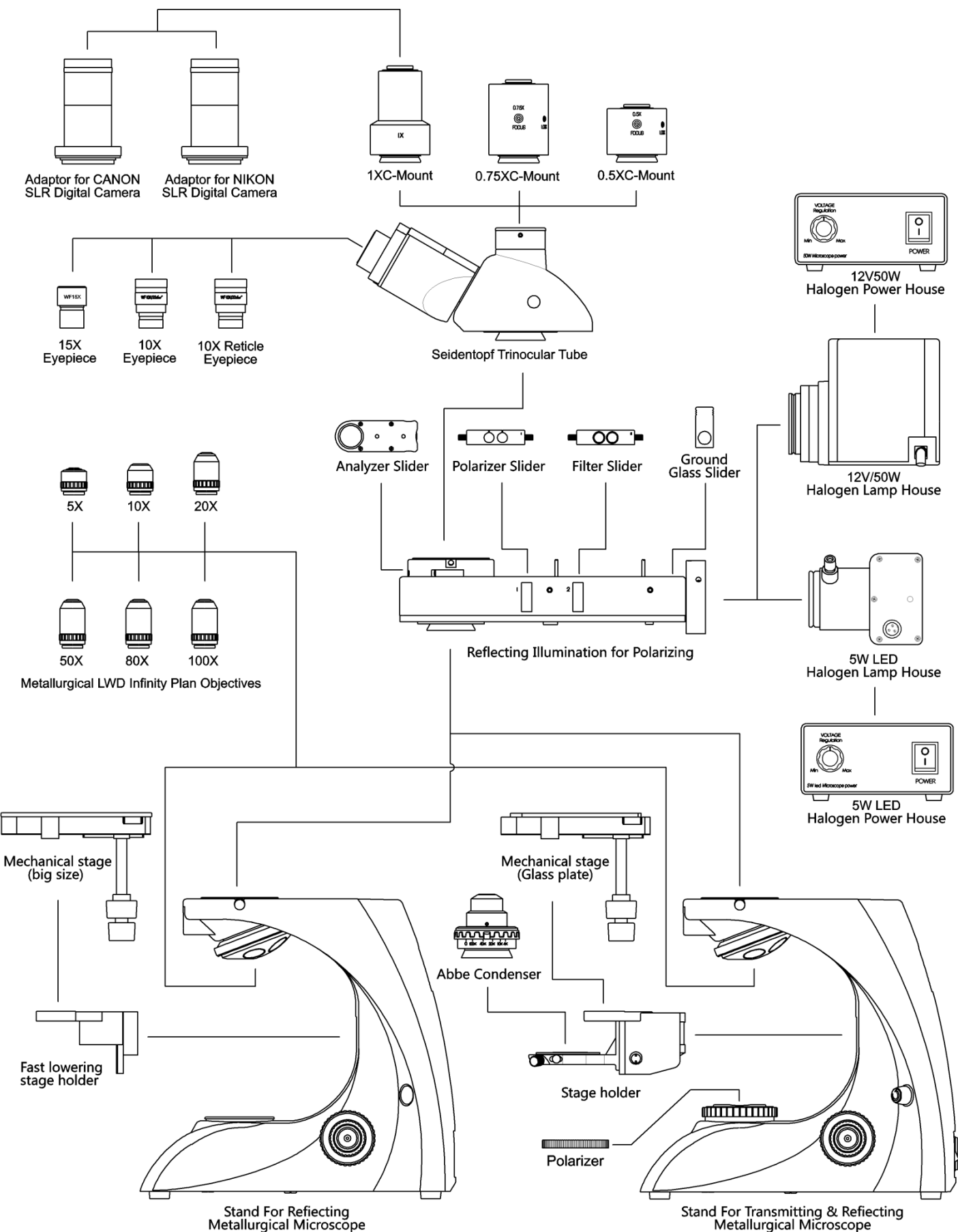
A13.2604-A/AD Metallurgical Microscope Reflect, BF/DF
