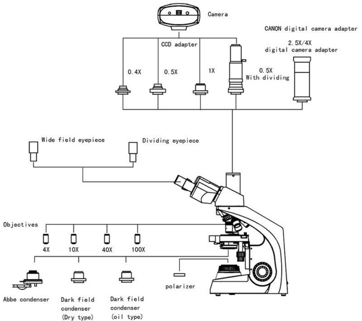
A12.0206 Laboratory Biological Microscope System Diagram
