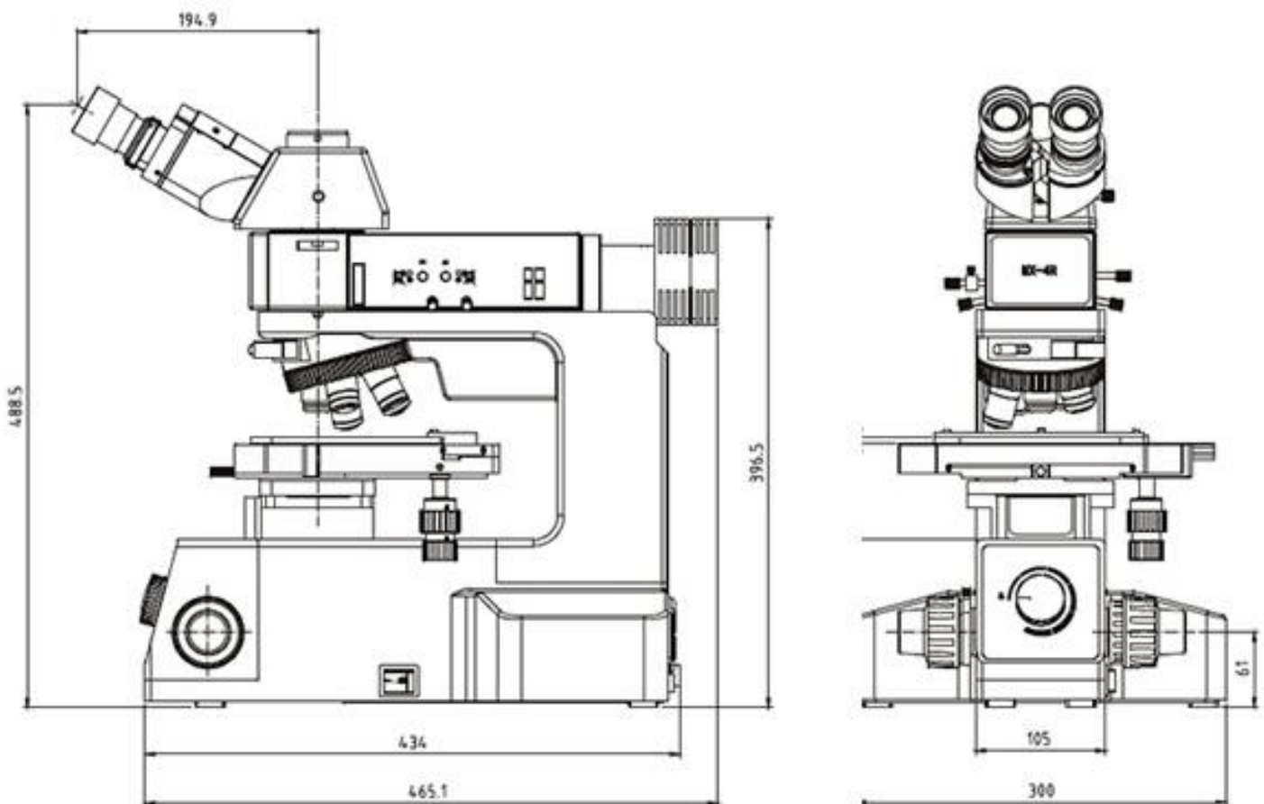
A13.0900 Metallurgical Microscope. System Dimension
