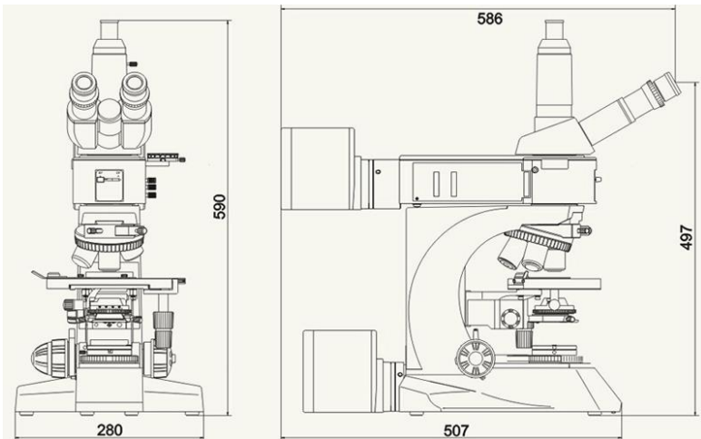
A13.1013 Metallurgical Microscope, BF/DF, PL, DIC
