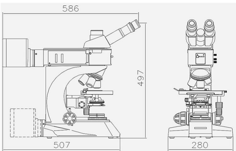
A13.1011 Metallurgical Microscope, BF/DF
