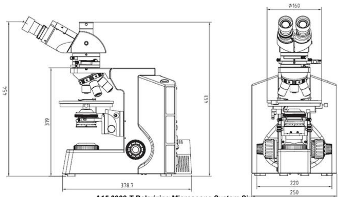
A15.0908-T Polarizing Microscope System Size
