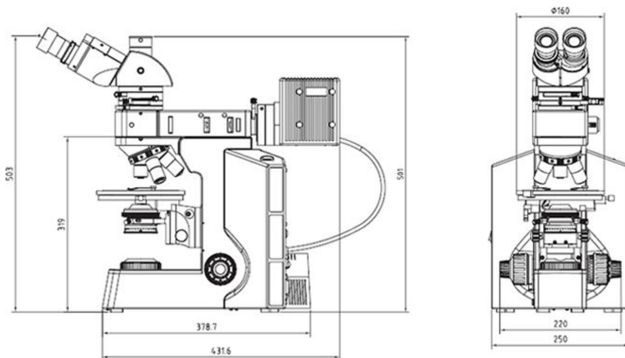
A15.0908-R,RT Polarizing Microscope System Size
