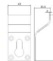
SB-301 SS Material: Stainless Steel 304 or 316 Finishing: SS, PSS, DAB, PVD
