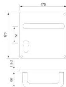
SB-100C-72 SS Material: Stainless Steel 304 or 316 Finishing: SS, PSS, DAB, PVD
