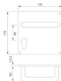
SB-100C-85 SS Material: Stainless Steel 304 or 316 Finishing: SS, PSS, DAB, PVD
