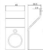
SB-300 SS Material: Stainless Steel 304 or 316 Finishing: SS, PSS, DAB, PVD
