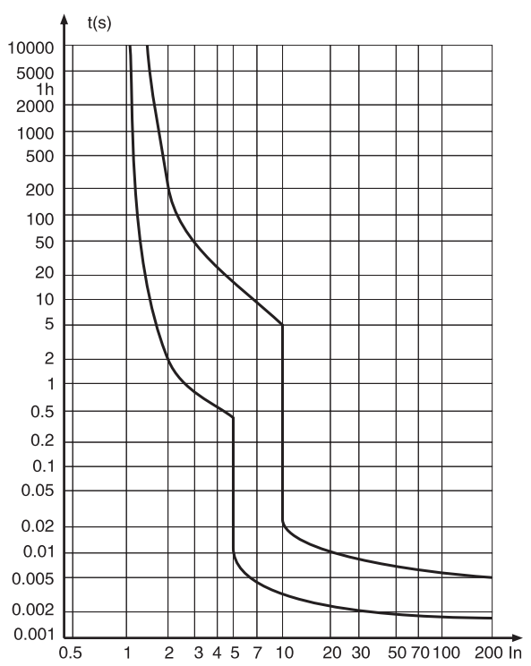
Diagram 2 Type C thermal/ electromagnetic tripping curve
