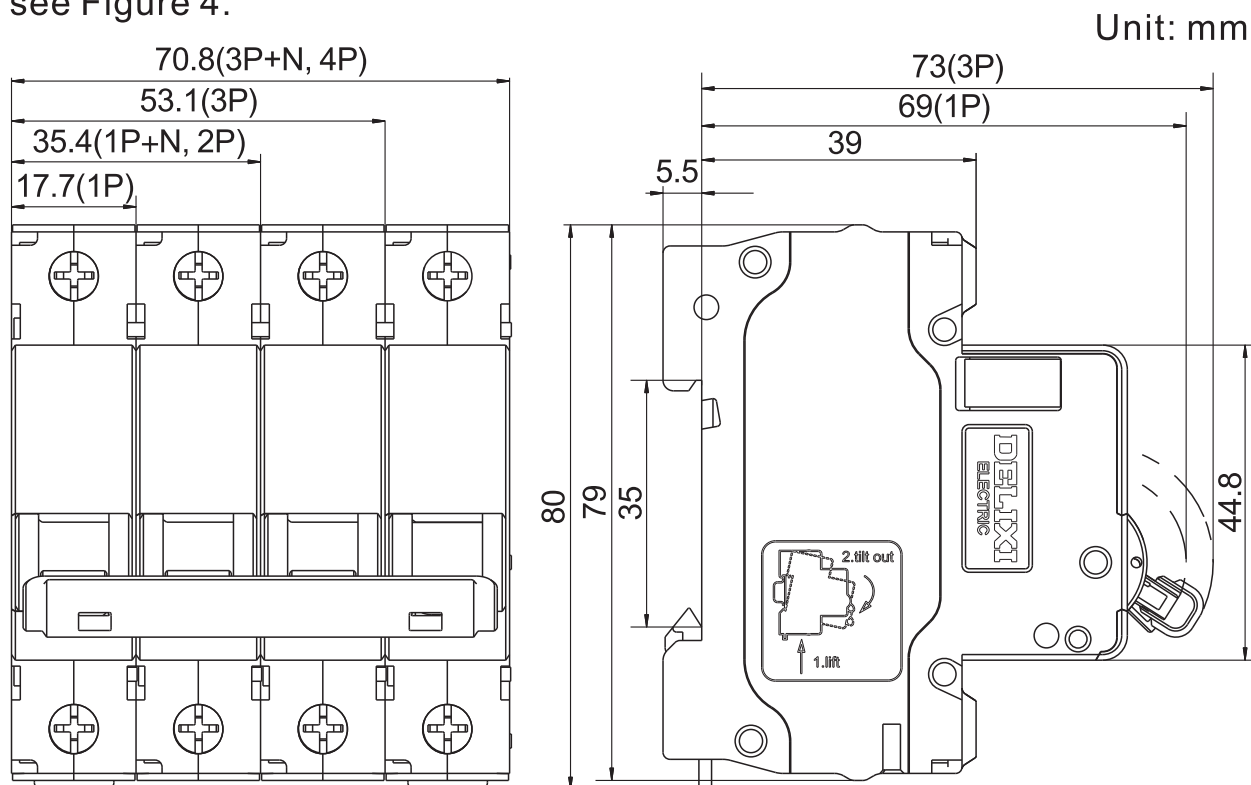
Figure 4. Overall and Installation dimensions
