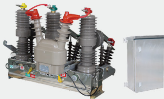
12kV Vacuum Circuit Breaker+ Recloser
