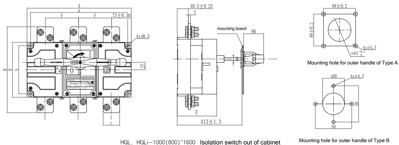
HGL、HGLi—1000(800)~1600 Isolation switch out of cabinet
