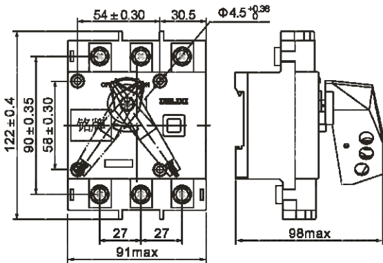
■ HGL、HGLi-80~100/3 Isolation switch
