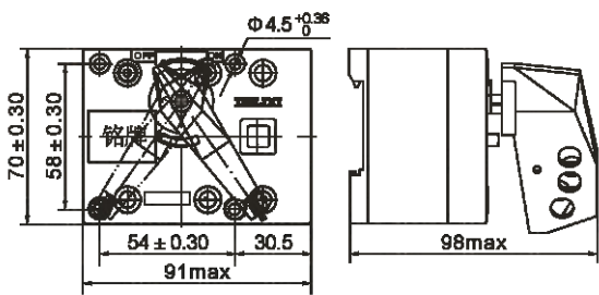
■ HGL、HGLi-80~100/3 Isolation switch
