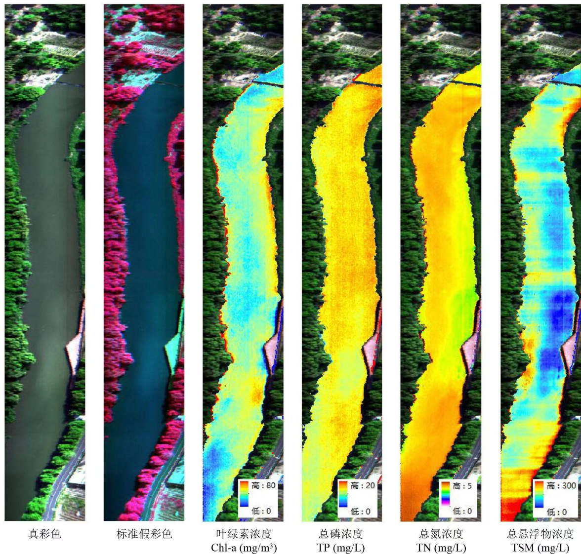
Figure 5 Inversion results of ATH9010-17 UAV hyperspectral river water quality detection data (Flight location: Xiamen City, Fujian Province, flight altitude: 100m; speed: 6m/s, wind speed: Level 2)
