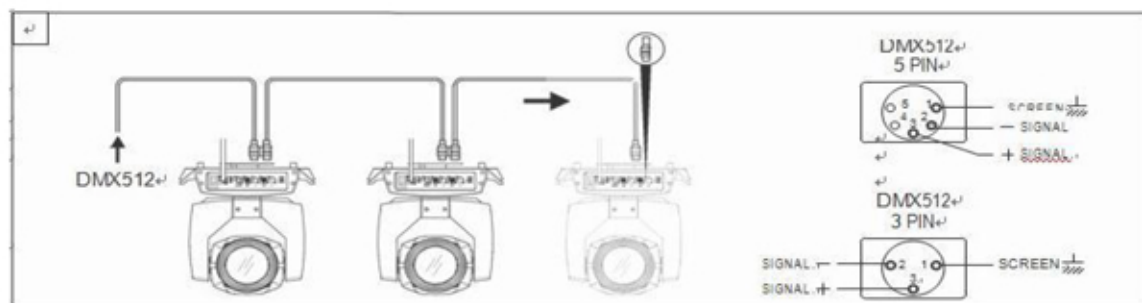
Pic1 DMX signal cable connection diagram
