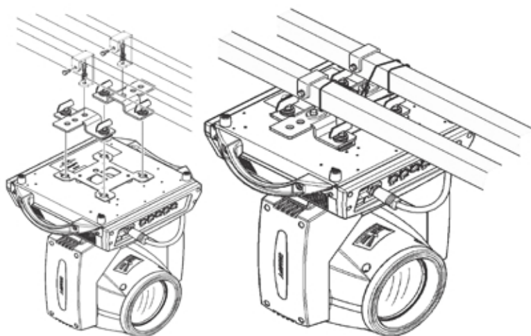
Pic2 Diagram of upside down luminaire
