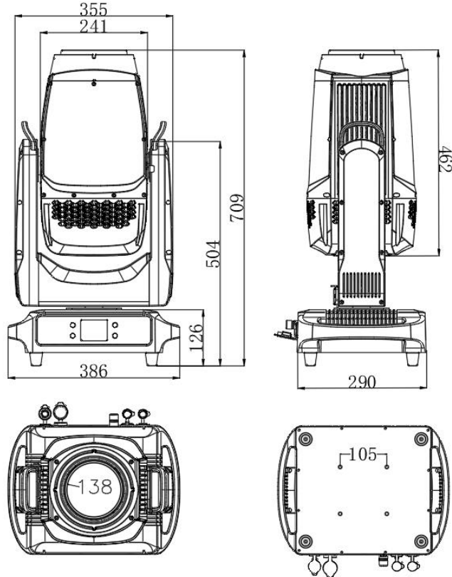
Product Dimension Drawing
