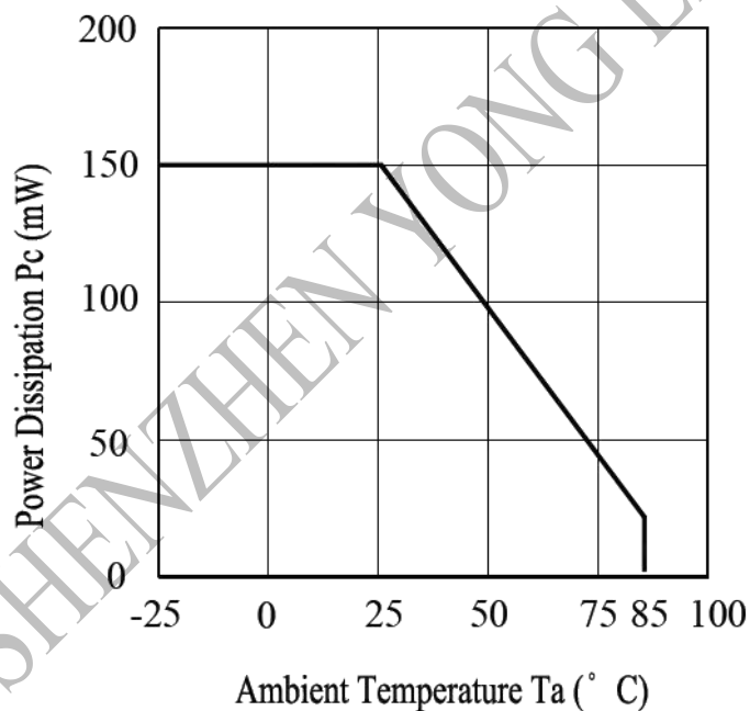
Power Dissipation VS. Ambient Temperature
