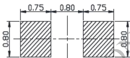
推荐焊盘尺寸 Recommended Soldering Pad
