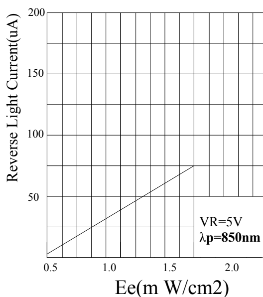
Reverse Light Current VS. Ee
