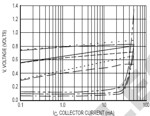
Figure 4. "ON" Voltages
