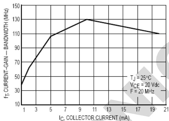
Figure 3. Current-Gain — Bandwidth
