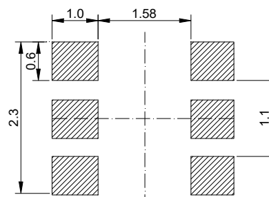
Recommended Soldering Pad
