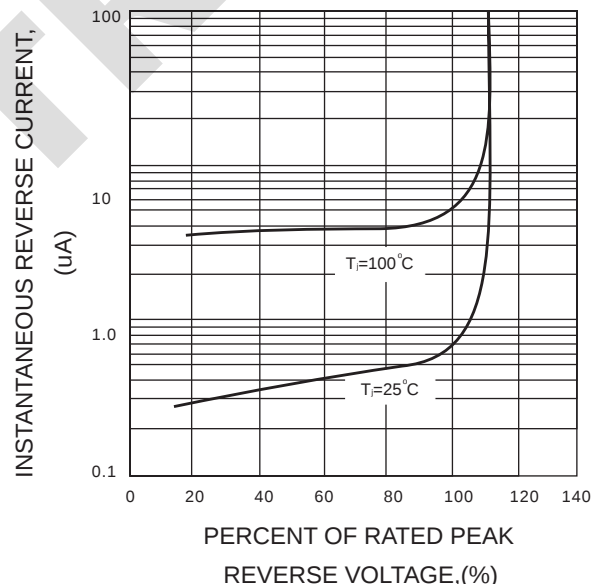
FIG.4-TYPICAL REVERSE CHARACTERISTICS
