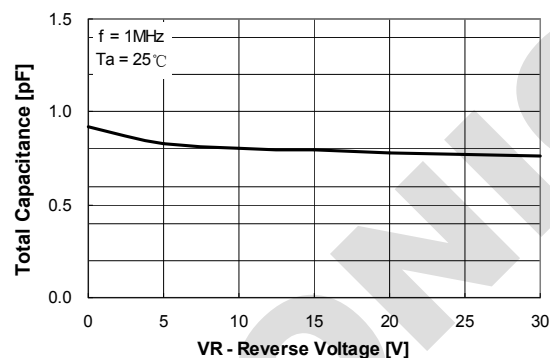
Figure 2. Total Capacitance
