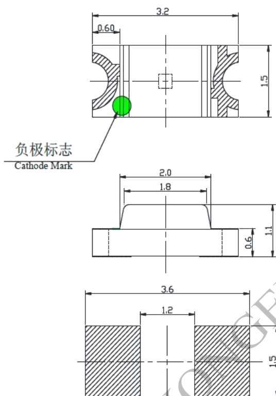
推荐焊盘尺寸 Recommended Soldering Pad
