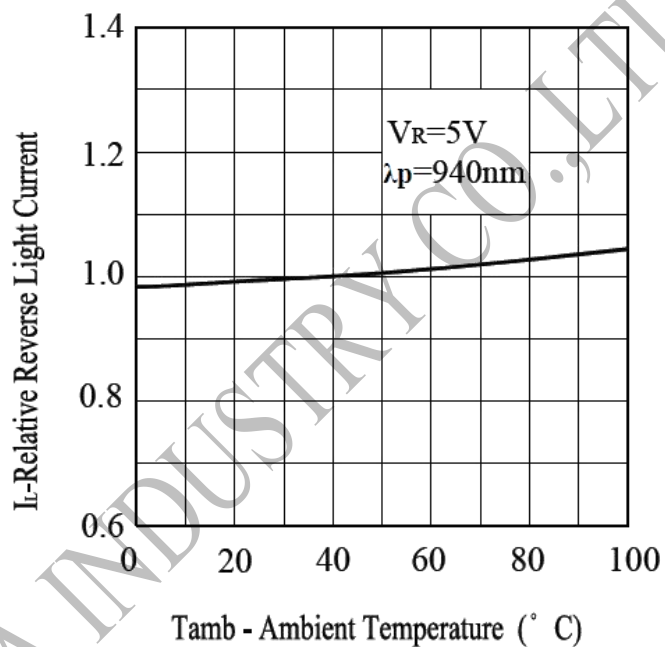
R_L -Relative Reverse Current VS. T_{amb} -Ambient Temperature
