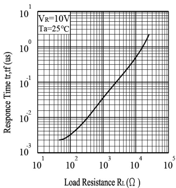
Response Time t_r, t_f VS. Load Resistance R_L
