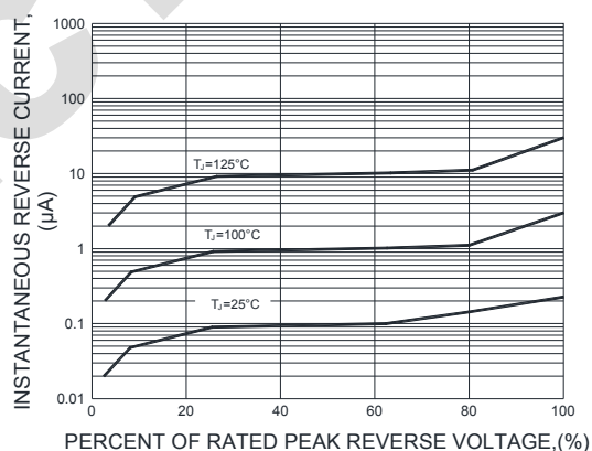
FIG.4-TYPICAL REVERSE CHARACTERISTICS
