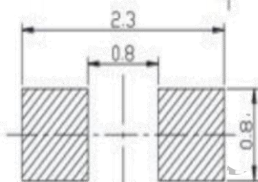
推荐焊盘尺寸 Recommended Soldering Pad
