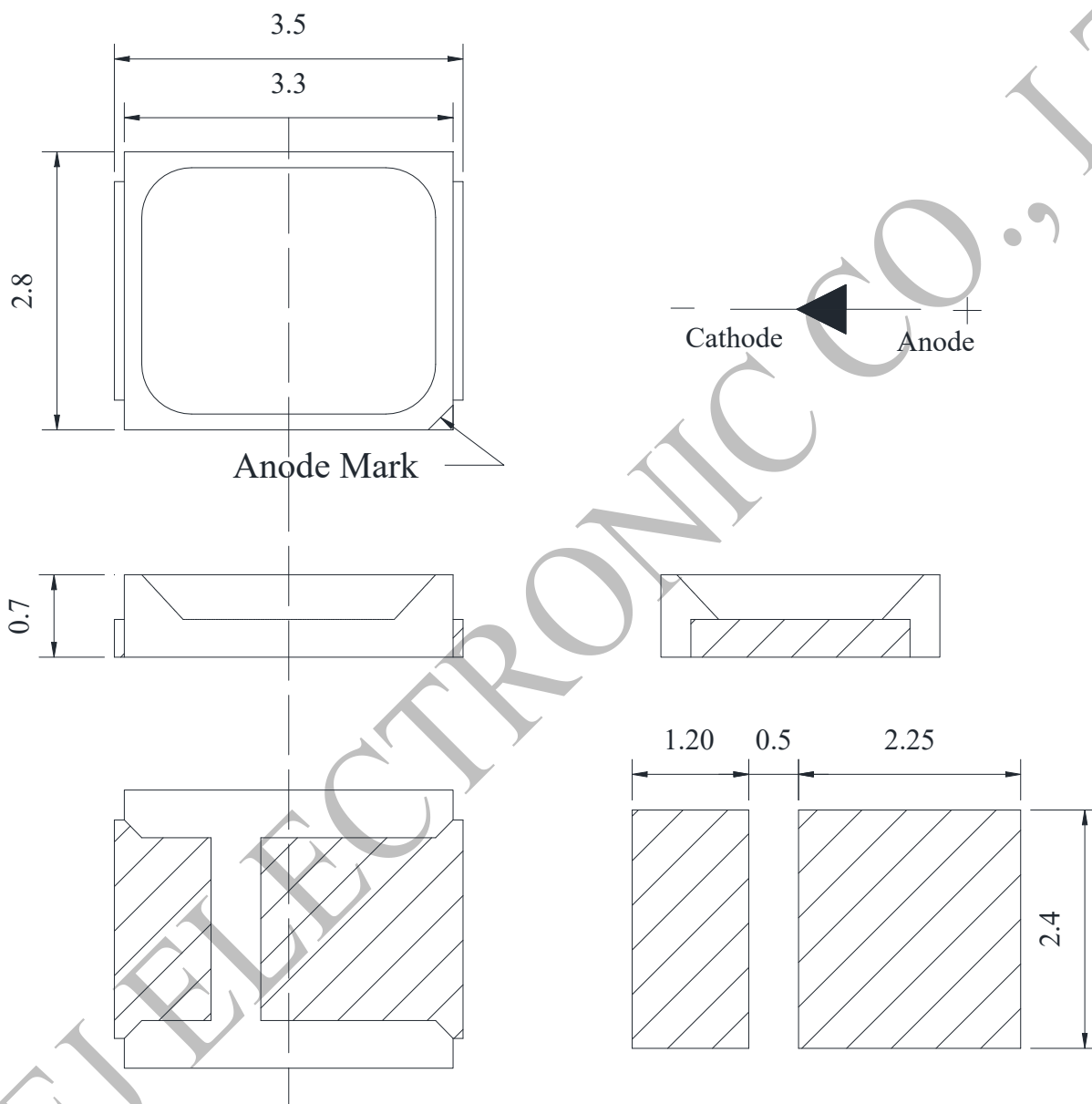
Recommended Soldering Pad
