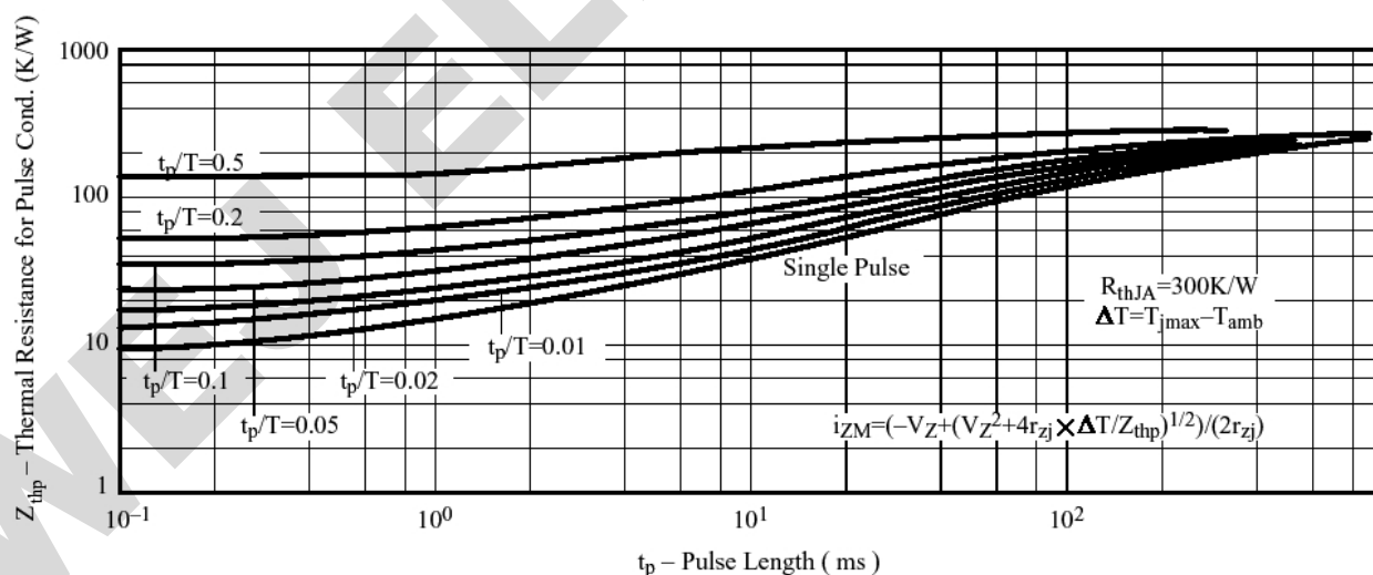
Figure 10. Thermal Response
