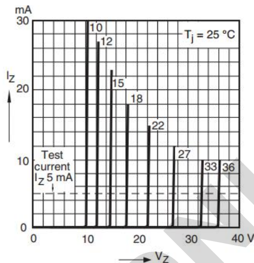
Fig.2-Zener Characteristic2
