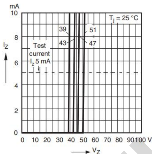
Fig.3-Zener Characteristic3
