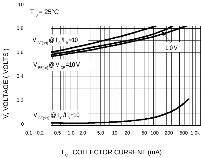
Figure 11. "On" Voltages
