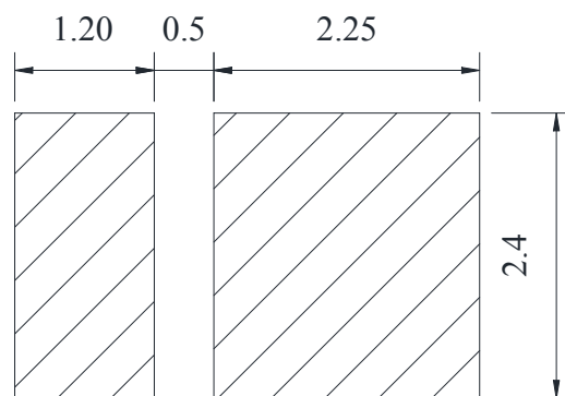
Recommended Soldering Pad
