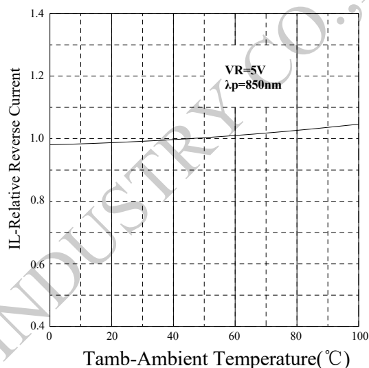
R_L -Relative Reverse Current VS. T_{amb} -Ambient Temperature
