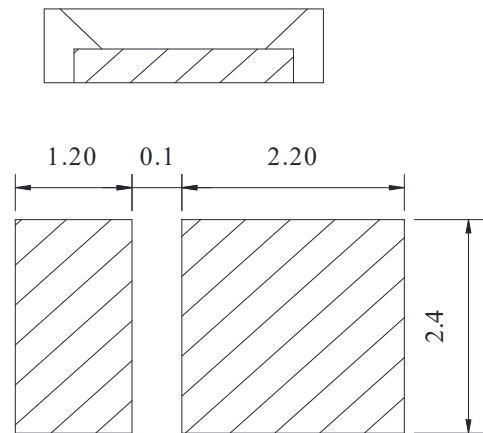
Recommended Soldering Pad
