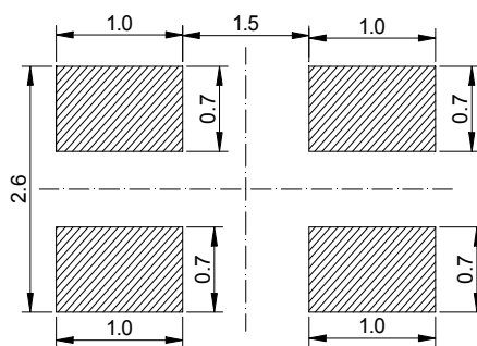
Recommended Soldering Pad
