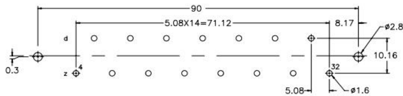
PCB LAYOUT(RECOMMENDED) (TOP VIEW TOL. :±0.05)
