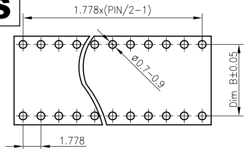
Recommended P.C.B Layout(Top Side)
