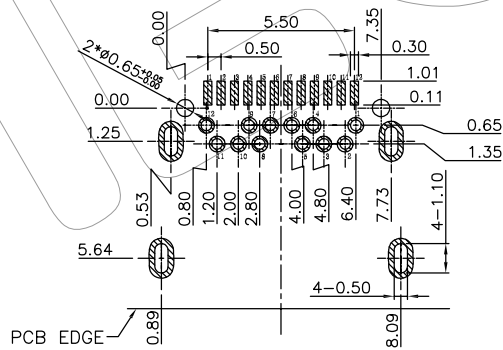
RECOMMEND PCB LAYOUT(TOLERANCE:±0.05) (THICKNESS:1.0mm OR 1.2mm)
