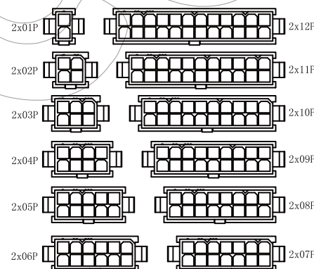
CIRCUIT SIZE LAYOUT
