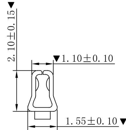
SEC C-C
