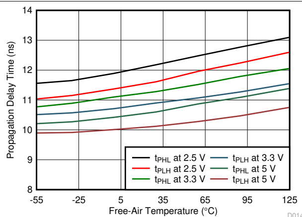
Figure 7-16. Propagation Delay Time vs Free-Air Temperature
