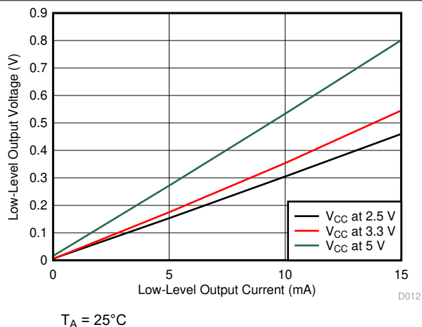
Figure 7-14. Low-Level Output Voltage vs Low-Level Output Current
