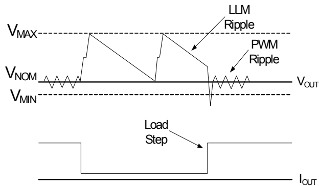
Figure 6: V_{OUT} Behavior in LLM Operation
