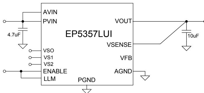
Figure 2: Typical Application Schematic.
