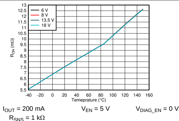
Figure 5. On Resistance ( R_{ON} ) vs Temperature
