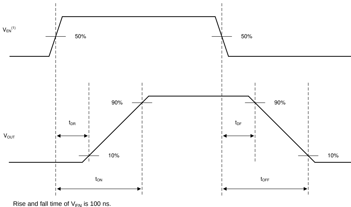
Figure 30. Switching Characteristics Definitions
