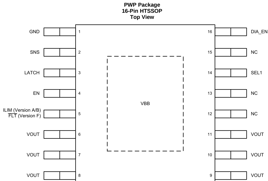
Pin Functions
