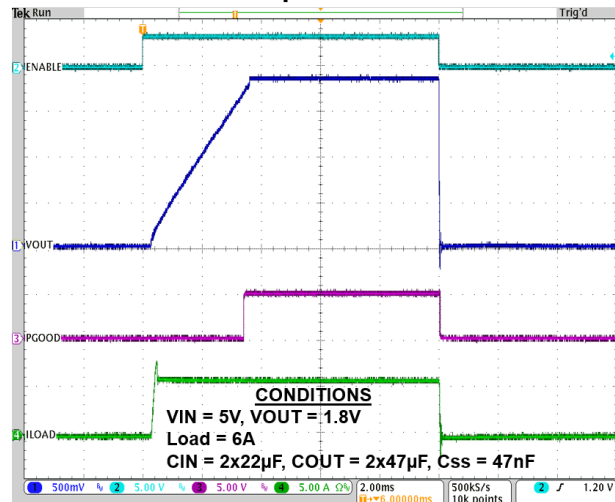
Startup Waveform
