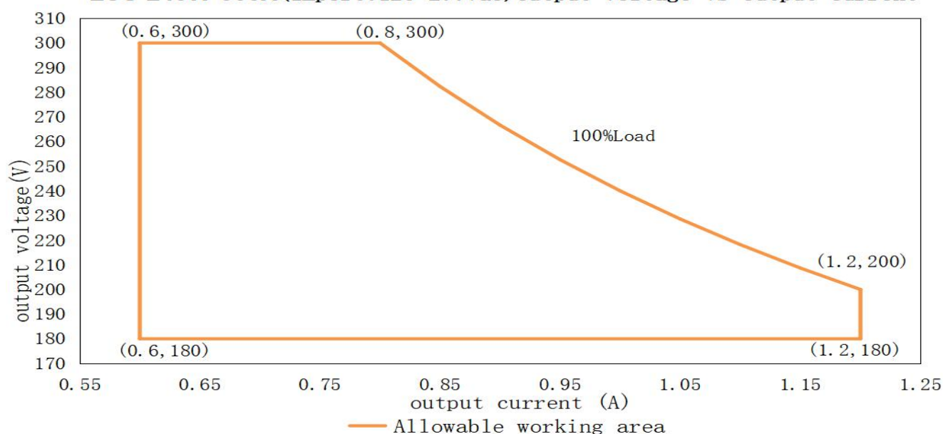
LCS-240W-300X (Import: 120–277Vac) output voltage VS output current
