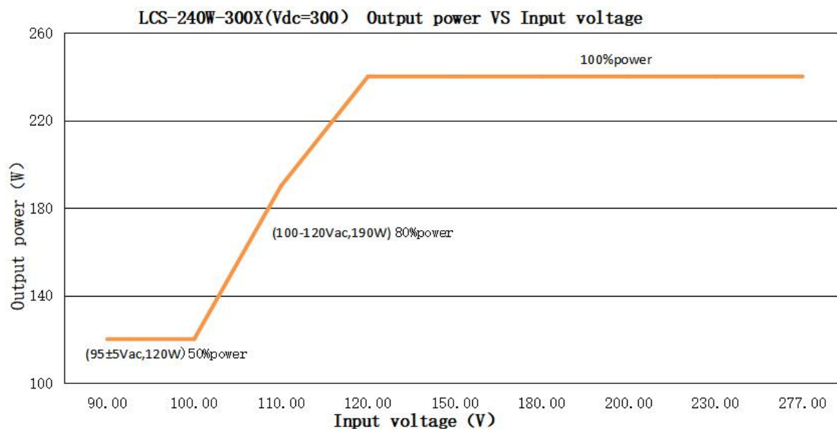
LCS-240W-300X(For output 300Vdc, the rated output current & power under different input voltage)
