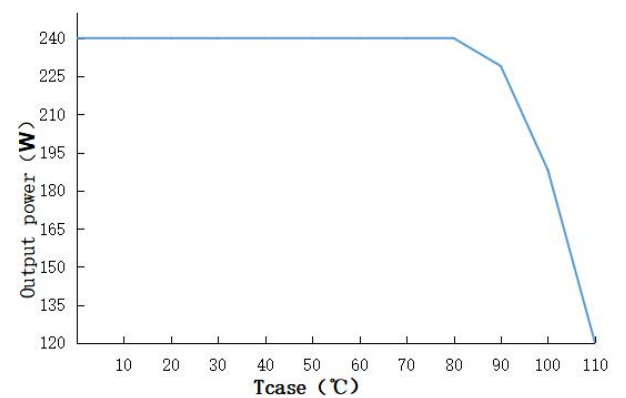
Output power VS Tcase
