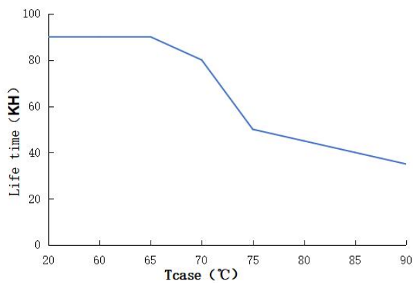
Tcase VS Life time
