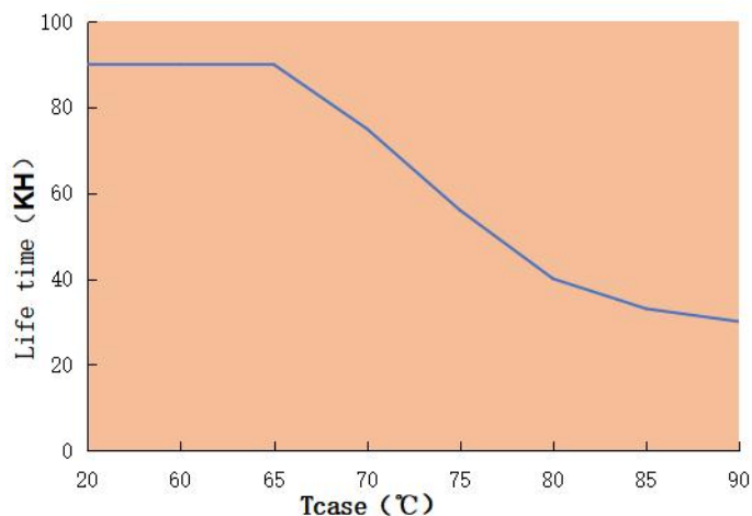
Tcase VS Life time (HVC-30W-56A/B)
