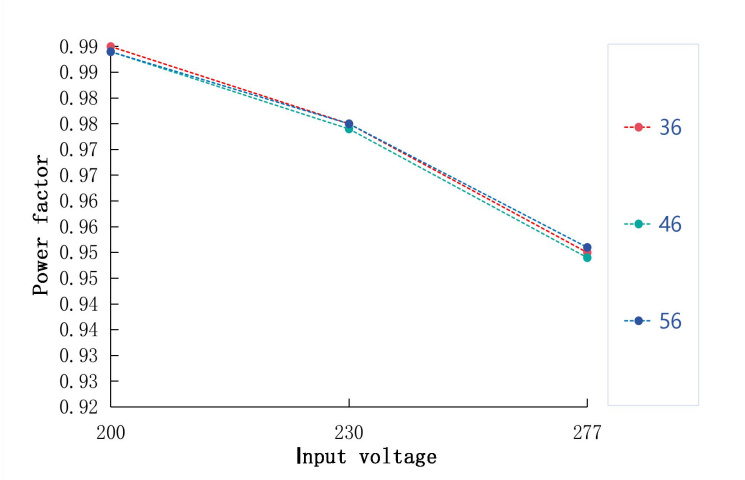
Power factor VS Input voltage
