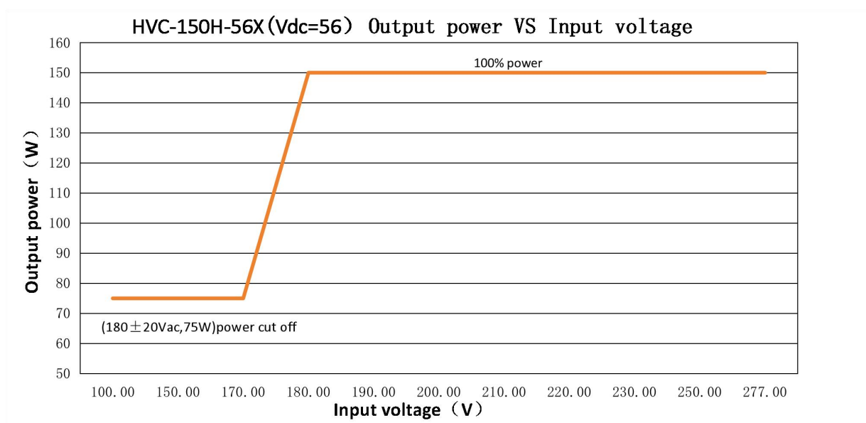
HVC-150H-56X(For output 56Vdc, the rated output current & power under different input voltage)
