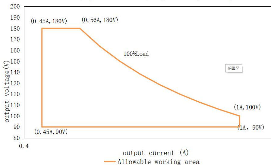
LDS-100W-180A/P/L (Import:120~277Vac) output voltage VS output current
