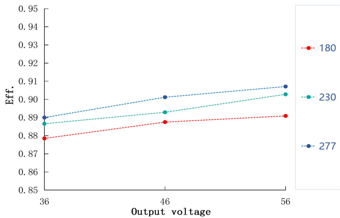
Eff. VS Output voltage
