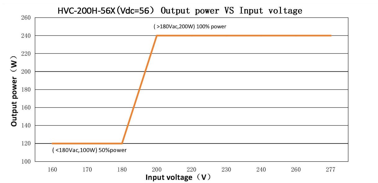
HVC-200H-56X(For output 56Vdc, the rated output current & power under different input voltage)
