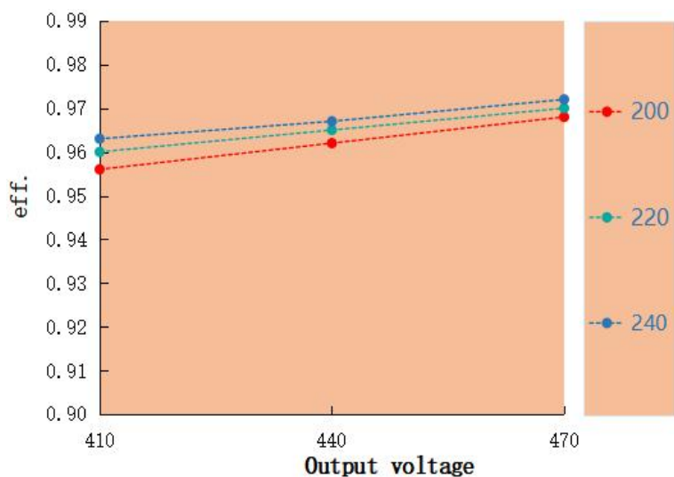
Eff. VS Output voltage LAG-120H-470A
