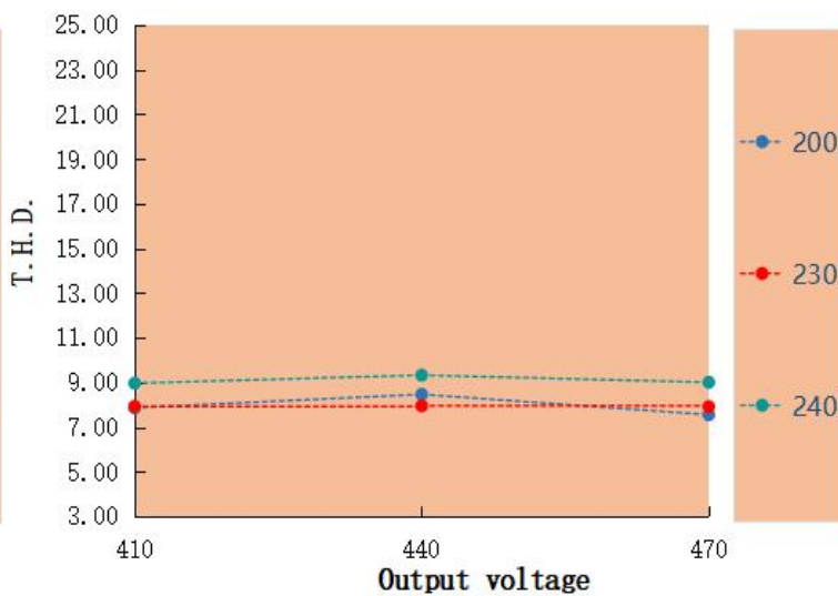
T.H.D. VS Output voltage LAG-120H-470A-XP
