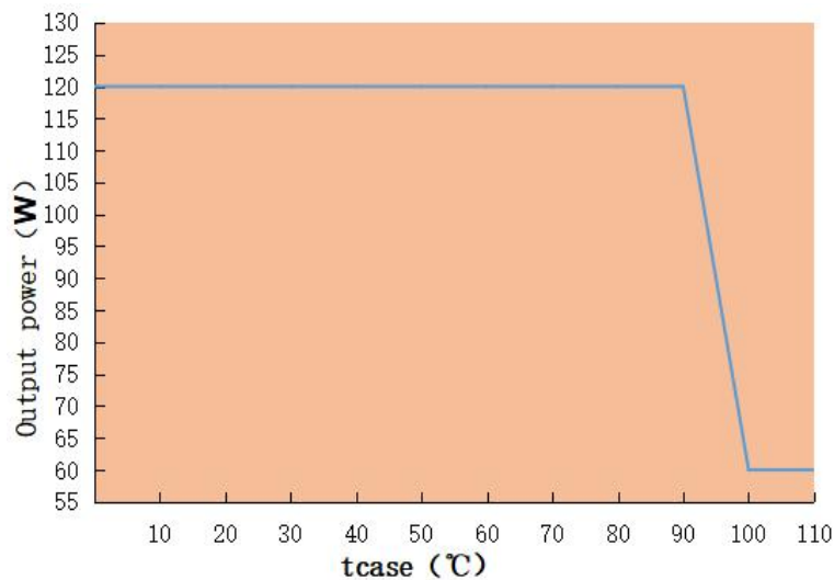
Output power VS Tcase LAG-120H-470A
