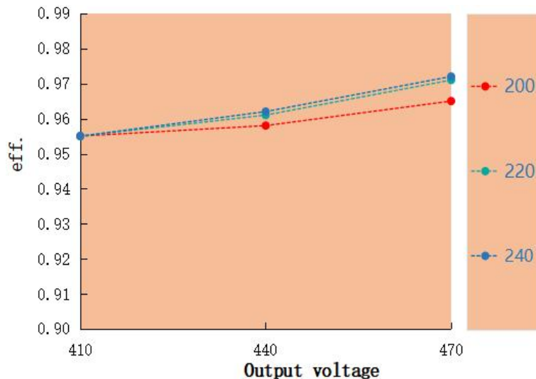
Eff. VS Output voltage LAG-120H-470A-XP
