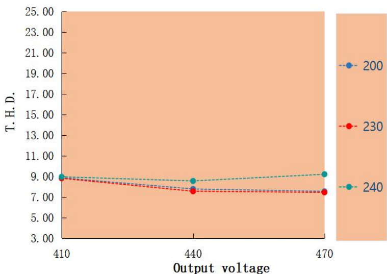
T.H.D. VS Output voltage LAG-120H-470A
